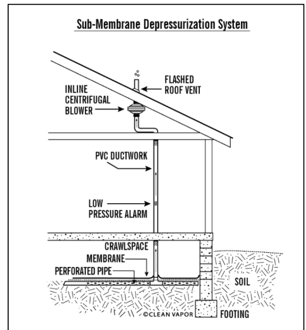
Figure 1. Typical sub-membrane depressurization system in a residential building (fan outside occupiable building envelope)
