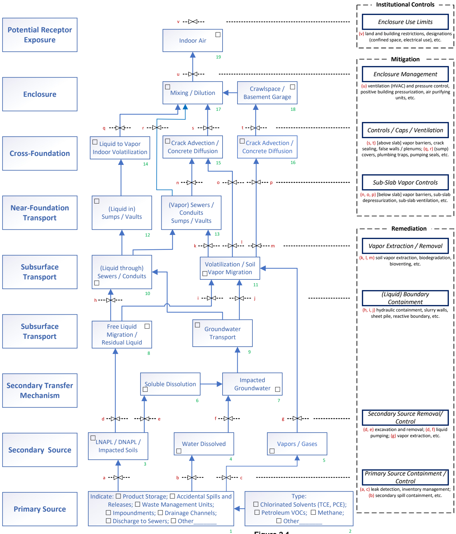
Figure 2-1. Flowchart for vapor intrusion mitigation conceptual site model development.
